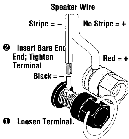
Figure 3. Reference 2000 speakers feature color-coded terminals. This example shows the most common way of connecting speaker wire by directly inserting into terminals.
